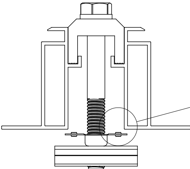
High-Lipped Module
