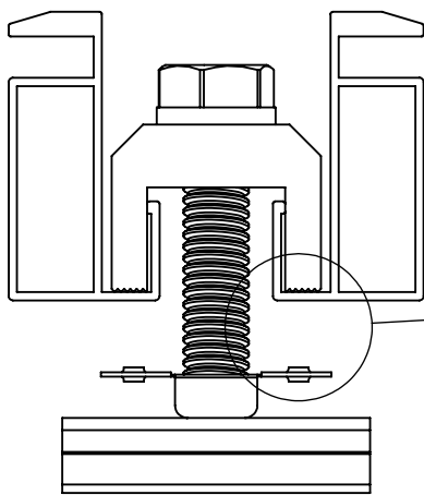
Low-Lipped Module
